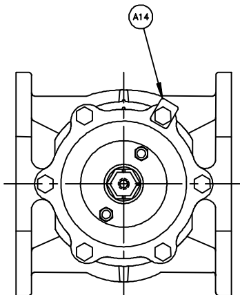
3.5 - 6 VALVES (SEE NOTE 4)
