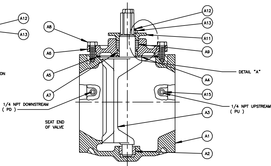
8.5 - 10 VALVES (SEE NOTE 4)
